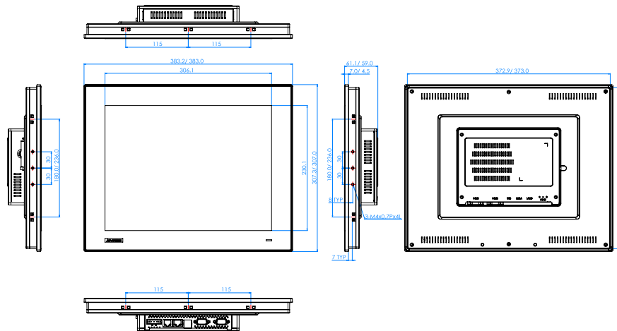
TPC-1551T/TPC-1551H Panel Cut-out Dimensions: 374.5 x 298.5 mm (14.74" x 11.75")
